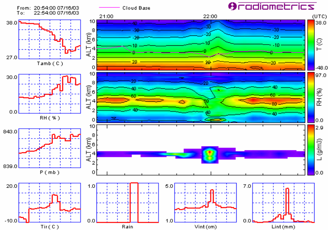
Figure 1 An example of MWRP operational screen output. Plots refer to data collected during 16 July 2003, in Boulder, Colorado, USA. A rain shower happened roughly at 22:00 UTC. Surface temperature, relative humidity, and pressure are shown on the left. Infrared cloud temperature, rain detection, integrated content of vapour and liquid are shown in the bottom. Contour plots show time-height cross sections of atmospheric temperature (top), relative humidity (middle) and liquid water (bottom).
