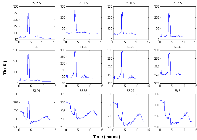
Figure 2 Time series of T_b observed by the MWRP twelve channels during 17 July 2003 in Boulder, Colorado. A rain shower occurred at 04:00 (elapsed time). For each channel, the corresponding frequency is shown on top (GHz).
