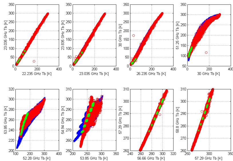
Figure 3 Rainfall spectral signature in terms of scatterplots between T_b at different frequencies. About one year of measurements are shown in red. Simulated data set are shown in blue, with non-raining cases evidenced in green.
