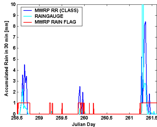
Figure 6 Same as Fig. 5. More rain events are shown.
