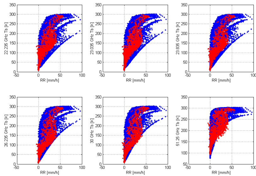
Figure 4 Scatterplots between Tb and rain rate. Simulations are shown in blue, while radiometric observations and respective rain rate estimates are shown in red.
