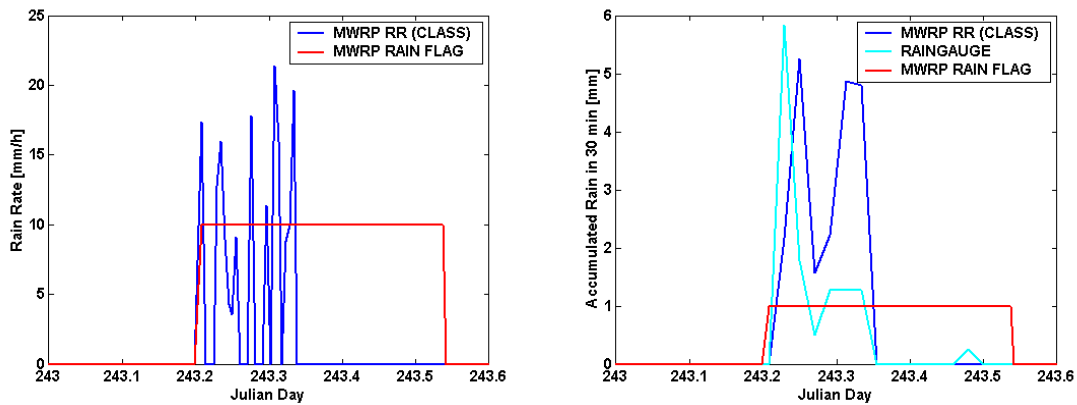
Figure 5 Left: Time series of MWRP estimated rain rate. Red line, representing rain sensor detection (0/1), has been multiplied by 10 for convenience. Right: Time series of 30-minute
