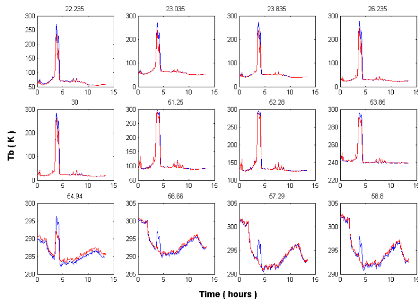
Figure 7 Same as Fig. 2, but considering two independent co-located MWRP units. The only difference between the operational and the development units is a special hydrophobic radome coating mounted on the latter. The operational observations are shown in blue, while observations with the coating are shown in red. The effects of the coating are evident for every channel, reducing T_b during rain. T_b differences range from about 60 K at 22.2 GHz channel to about 4 K at 58.8 GHz channel.
