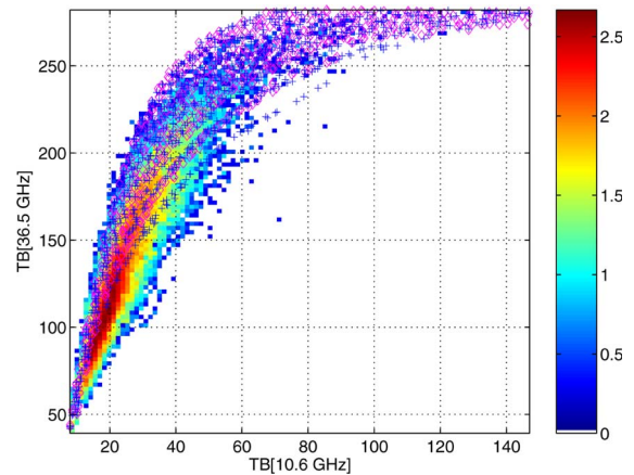
Fig. 5. (Crosses and diamonds) Simulated and measured T_B 's for the 10.6- and the 36.5-GHz frequencies at 30^\circ elevation angle. The color scale accounts for \text{Log}_{10} of the number of occurrences.
