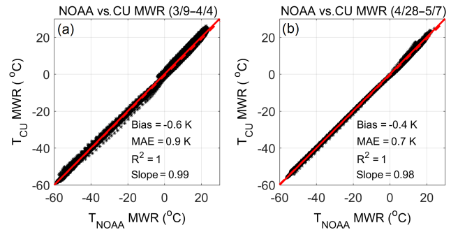
Figure 2. Comparison between temperature observed by CU MWR and NOAA MWR between (a) 9 March–4 April and (b) 28 April–7 May, 2015. The missing days in April coincide with the failure of the NOAA MWR surface sensor. A 1-to-1 line is indicated in solid red, and the regression is shown by the dashed red line.
