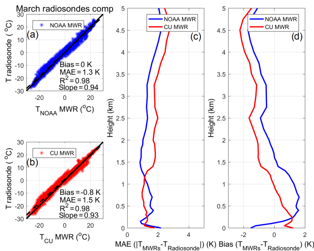
Figure 3. MWRs vs. radiosonde comparison of T for 9–19 March including 38 radiosonde launches: (a–b) one-to-one comparisons between T observed by the radiosondes and the (a) NOAA and (b) CU MWR between the surface and 5 km a.g.l. One-on-one line is indicated as a solid black line and the regression as a dashed black line. (c–d) Vertical profiles of MAE and bias for the same variable for the NOAA MWR (blue line) and CU MWR (red line).
