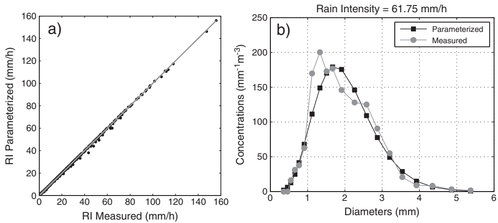
Fig. 2. Parameterized rain rate against measurements. The line represents the perfect linear fit (1 × 1).
