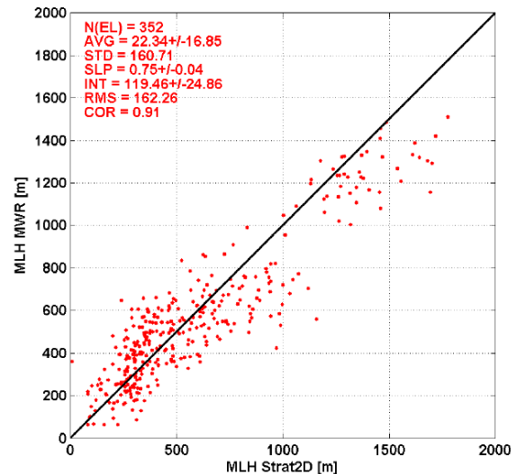
Figure 2. Scatter plot of 1-hour averaged MLH derived from MWR (Y-axis) and Strat2D (X-axis) for March 2012 at the SIRTA site. Number of elements (N(EL)), average X-Y difference (AVG), standard deviation (STD), root-mean square difference (RMS), correlation coefficient (COR), slope (SLP) and offset (INT) of a linear fit are included. N(EL), SLP, and COR are dimensionless, while AVG, STD, RMS, and INT are in meters.
