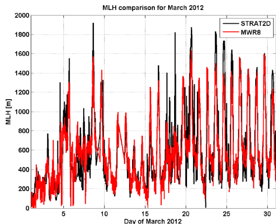
Figure 1. Time series of MLH derived from MWR (red line) and from STRAT2D algorithm (black line) for March 2012.
