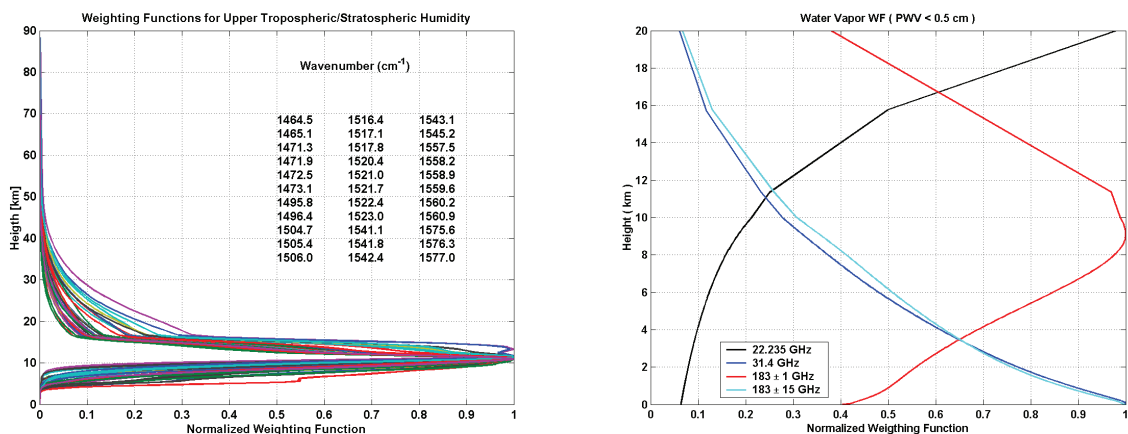
Figure 3: Normalized Weighting Functions for AIRS UTH sounding channels (left) and selected MWRP and GSR channels (right).
