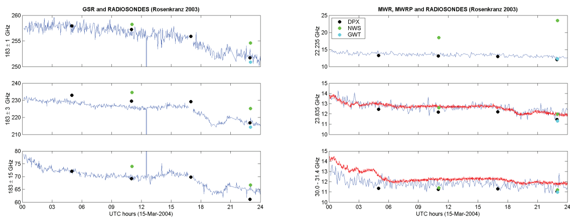
Figure 4: 24-hour time series of simulated and measured T_b at selected GSR, MWR, and MWRP channels.
