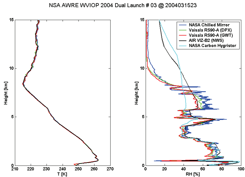
Figure 1: A case of multi-radiosonde launch. Three out of five radiosondes were attached at the same balloon and launched from DPX, while the other two were launched at NWS and GWT sites.
