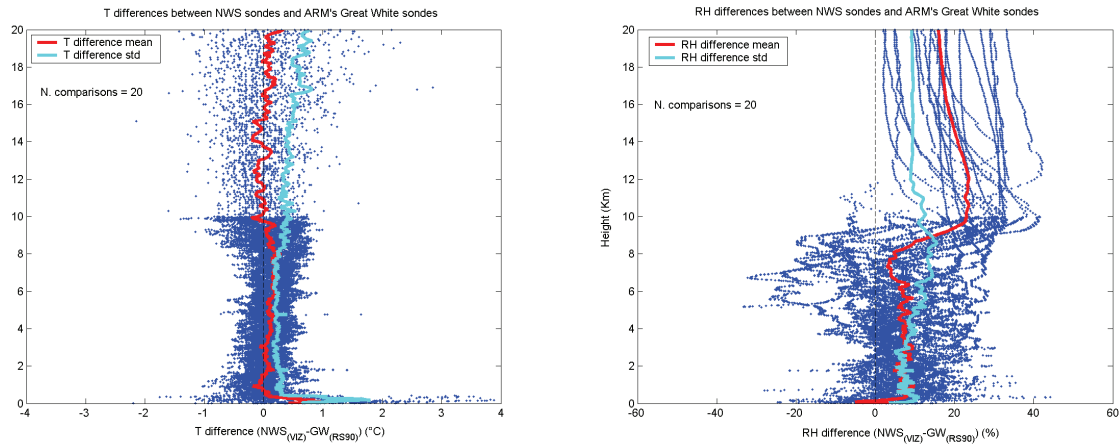
Figure 2: Difference in temperature (left) and relative humidity (right) profiles for the entire set of simultaneous soundings launched at NWS and GWT sites (blue dots). Mean value (red line) and standard deviation (cyan line) are also displayed.
