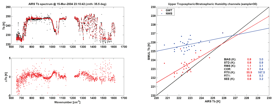
Figure 5: Left: Measurements (black) and NWS simulations (red) of AIRS Tb spectrum. The difference between the two is shown in the bottom panel. Right: scatter plot and statistics of simulated (blue: NWS; red: GWT) minus measured Tb considering only AIRS UTH channels.
