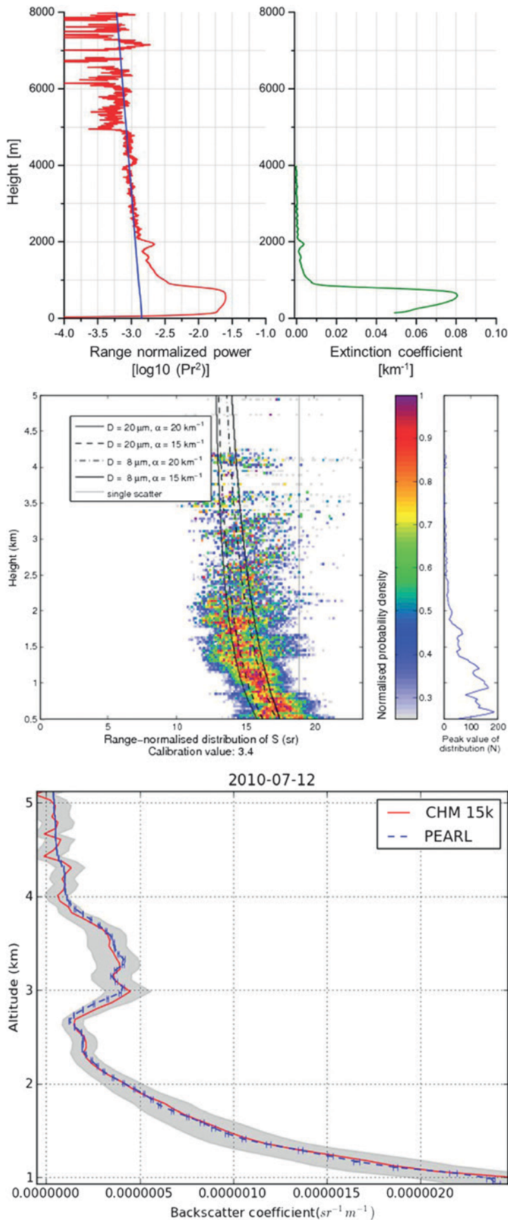
FIG. 4. (top) Automatic lidar and ceilometer calibration techniques. (left) Use of the near-infrared molecular attenuated backscatter at 3–4-km height integrated for 2 h (signal in red, theoretical attenuated molecular profile in blue). The observed profile has been scaled to match the known attenuated molecular profile. (right) The extinction profile (green) scaled so that it matches the integrated aerosol optical depth derived from a collocated sun photometer. (middle) Calibration technique for the water cloud extinction method, relying on the integrated attenuated backscatter return for single scattering being equal to the reciprocal of twice the liquid ratio S . The dotted line is the theoretical value of S = 18.8 \pm 1 sr for cloud water droplets at 910 nm. For most ceilometers a range-dependent correction for multiple scattering must be applied (solid and dashed lines). In this example the factory calibration has been adjusted by a factor of 3.4, so that the value of S derived from observed integrated backscatter return over one month agrees with the theoretical predictions. Also shown is the number of individual profiles containing suitable liquid clouds used for the calibration as a function of the height of the cloud. (bottom) Independent evaluation of the molecular calibration technique for a Jenoptik CHM15K ceilometer operating at 1064 nm by comparison with a collocated lidar system having a much more powerful laser at the same wavelength.
