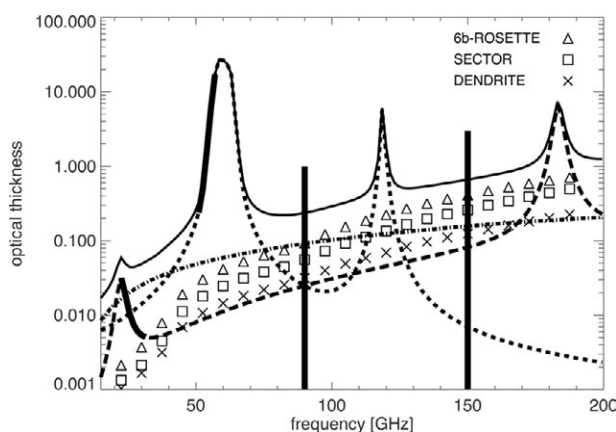
FIG. 2. Microwave spectrum: total optical thickness (bold) as a function of frequency calculated for a winter condition at UFS (surface temperature \sim 270 \text{ K} and IWV \sim 4 \text{ kg m}^{-2} ). The assumed LWP is 0.1 \text{ kg m}^{-2} , whereas the SWP is set to 0.3 \text{ kg m}^{-2} . An exponential size distribution for the snowflakes is assumed (see text). The dotted line shows the contribution due to oxygen, the dashed line shows the contribution due to water vapor, and the dotted-dashed line shows the contribution due to liquid water. The different symbols indicate the resulting optical thickness due to the snow, assuming different snow particles according to Liu (2008b). The thick black lines show the measurement range of the microwave radiometers.
