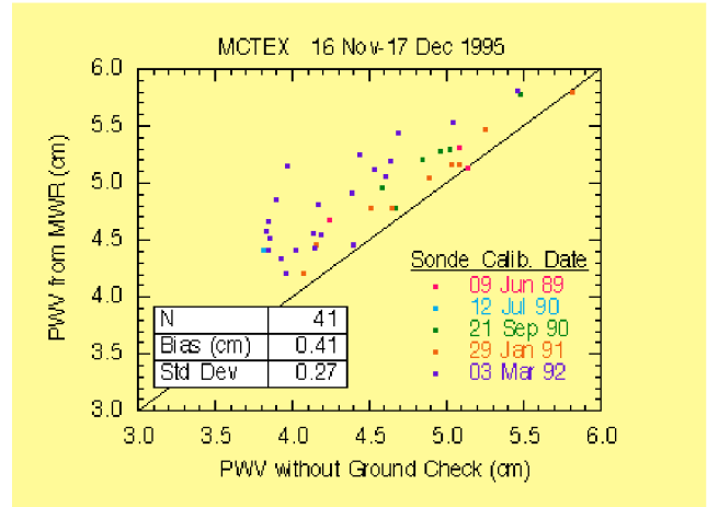
Figure 5. Scatter plot of PWV from the microwave radiometer compared with integrated soundings after removing the ground check corrections.
