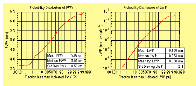
Figure 2. Probability distributions of PWV and LWP.
