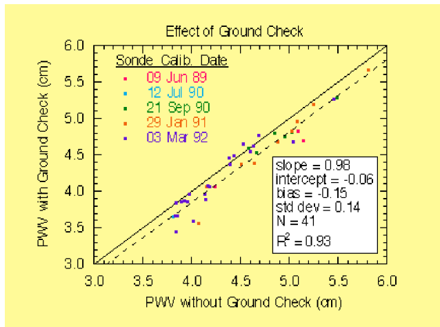
Figure 4. Scatter plot of integrated water vapor from soundings with and without the effect of the calibration ground check.
