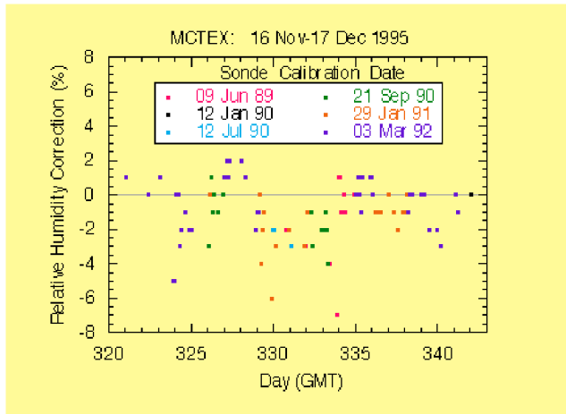
Figure 3. The time series of relative humidity corrections coded by sonde calibration date.
