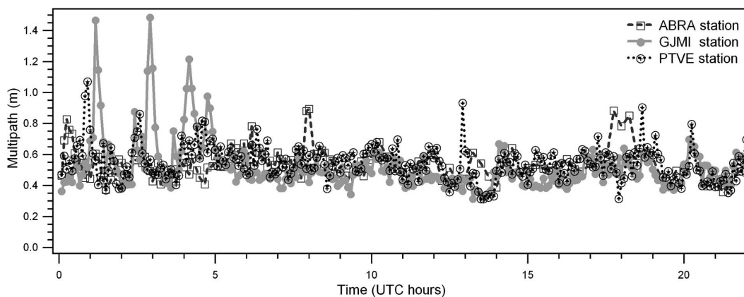
FIG. 10. Mean of multipath in the GPS signal in the three RACCI GPS stations (6 Oct 2002).
