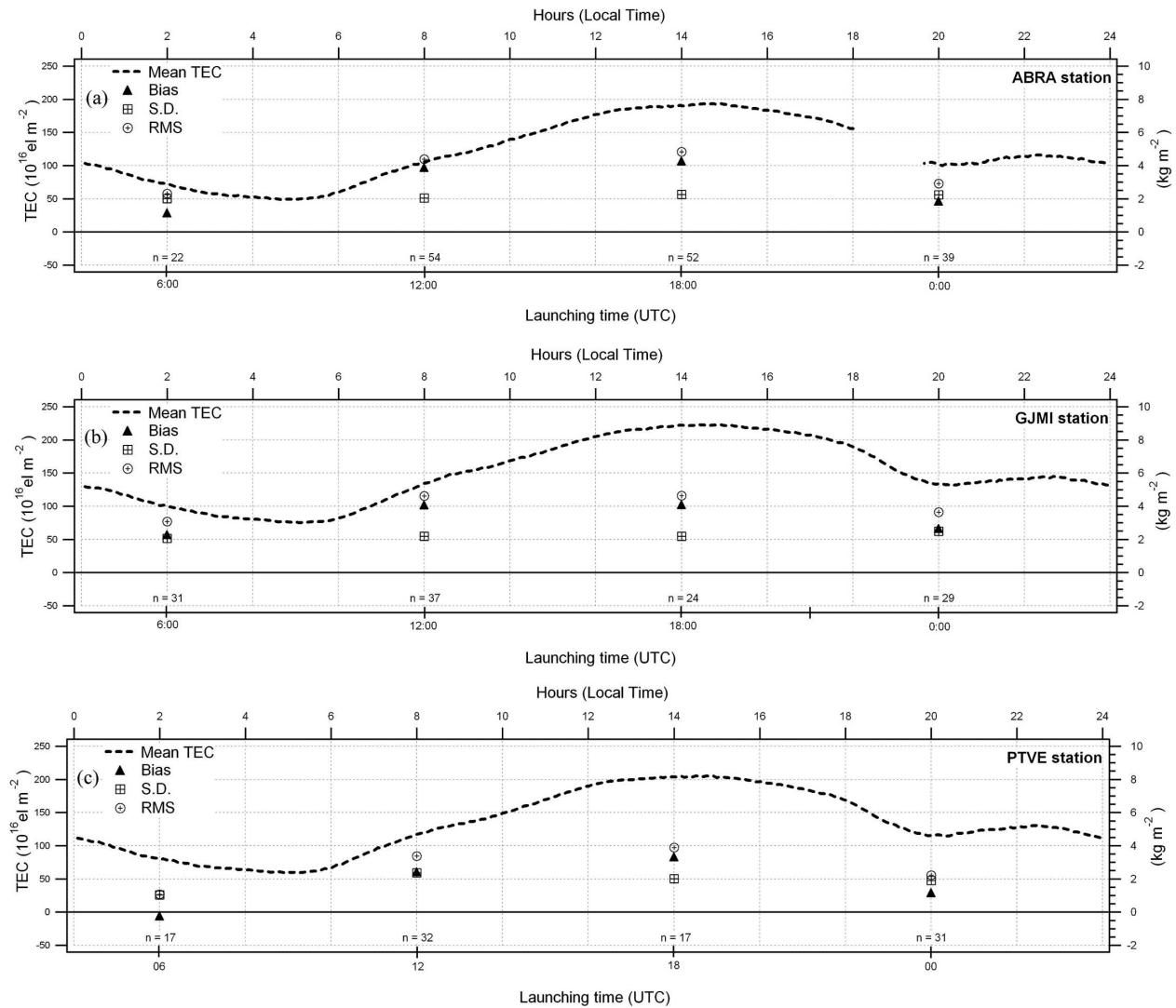
FIG. 9. The line-of-sight TEC average as a function of LT and statistical measurements of the comparison between the GPS and RS80 in function radiosonde launching synoptic time.
