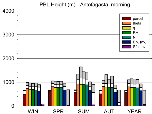
Figure 7. Same as Figure 5 but for Antofagasta, Chile (22°S, 137°W), for morning only.
