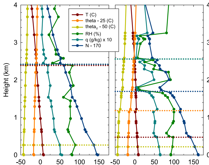
Figure 3. Planetary boundary layer height estimates using six methods for Lerwick, United Kingdom, for (left) 1100 UTC 17 February 2007 and (right) 2300 UTC 23 December 2006. Profiles include temperature, potential temperature ( \Theta ), virtual potential temperature ( \Theta_v ), relative humidity, specific humidity, and refractivity ( N ), some shifted for clarity. Estimated PBL heights are shown by dashed horizontal lines. These soundings do not indicate the presence of surface-based inversions.
