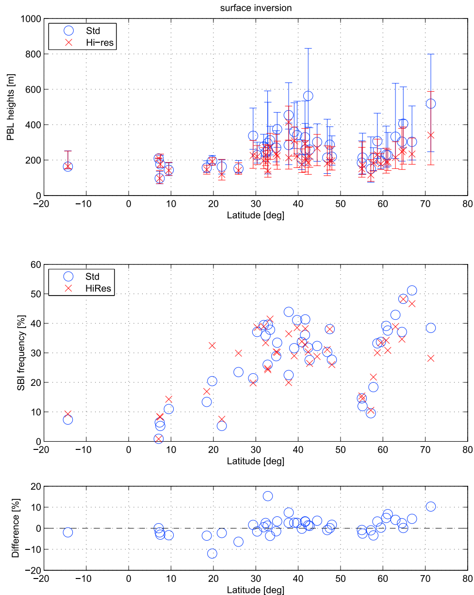
Figure 11. (top) Same as Figure 10, but showing results for the height of the top of surface-based inversions (SBI). (middle) Frequency (%) of SBI occurrence based on standard (blue) and high vertical resolution (red) data. (bottom) Difference (standard minus high resolution) in SBI frequency.
