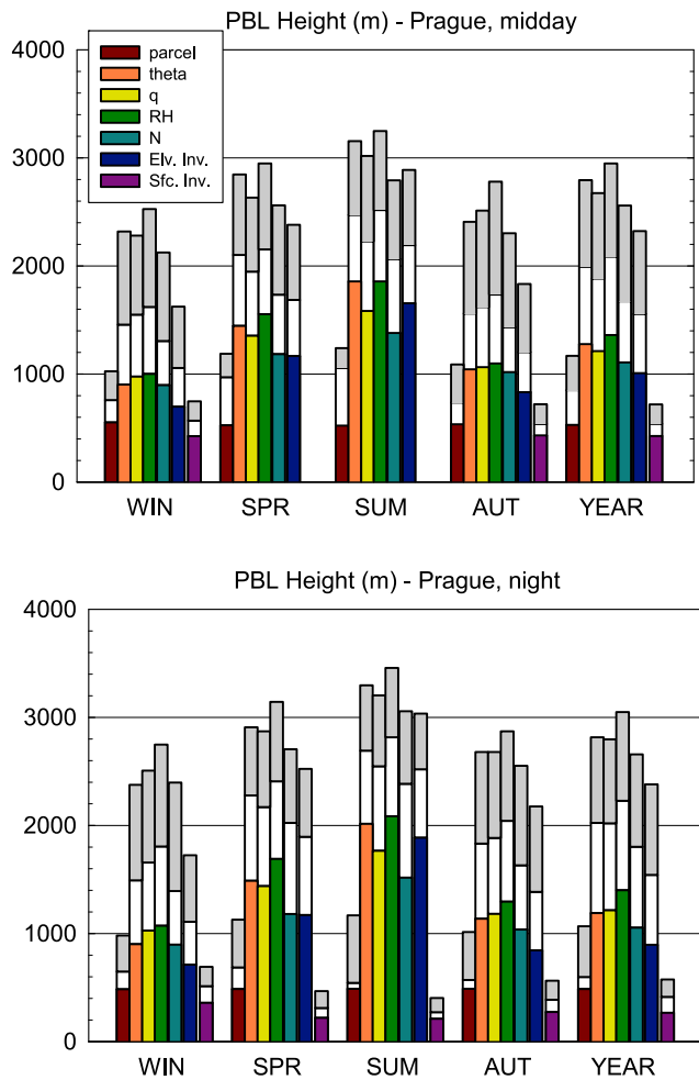
Figure 5. Seasonal and annual quartile values of planetary boundary layer height (m above ground level) at Prague, Czech Republic (50°N, 14°E), based on data for 1999–2008. For each method, the 25th, 50th, and 75th percentile values are shown (in colored, white, and gray bars, respectively), for (top) midday and (bottom) nighttime. Heights based on surface-based inversions are from a different set of soundings than heights based on the other methods. They are not shown for daytime at Prague because they occur rarely (1% of soundings).
