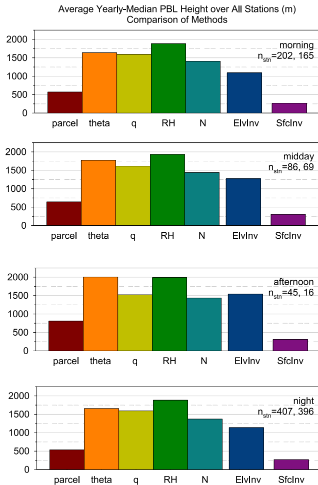
Figure 4. Average values (over all stations) of yearly median planetary boundary layer heights estimated using seven different methods. (top to bottom) Results for morning, midday, afternoon, and nighttime (see text for details). The number of stations used to compute each average ( n_{\text{stn}} ) is shown; the first value applies to six methods and the second applies to surface-based inversions.
