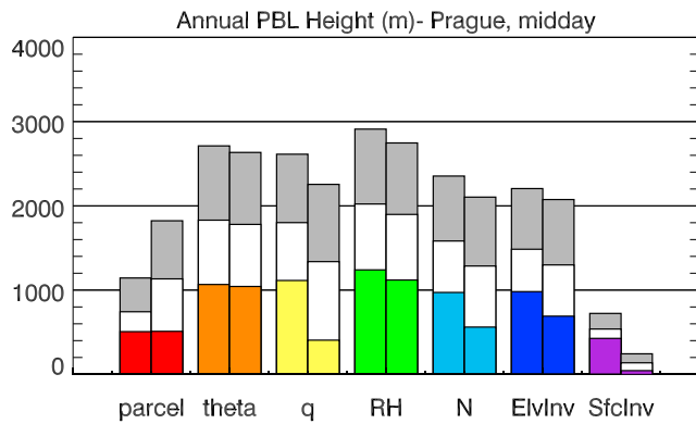
Figure 12. Effect of surface-level observations on climatological annual PBL height estimates at Prague, Czech Republic (50°N, 14°E), based on data for 1999–2008. For each PBL height estimation method, 25th, 50th, and 75th percentile values of PBL height (m) are shown based on calculations excluding (bars on left) and including (bars on right) surface data. The results excluding surface data are as in Figure 5, top.
