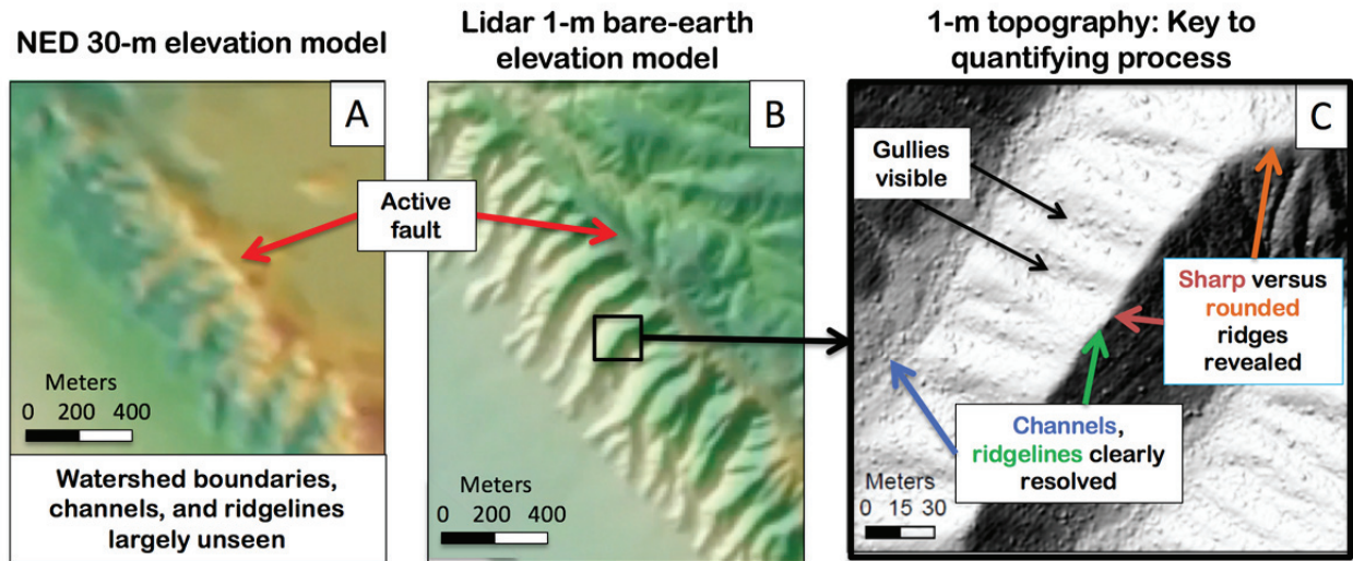
FIGURE 10.17 (A) A shaded-relief image of a portion of the Dragon’s Back Pressure Ridge derived from the 30-m-resolution National Elevation Dataset (NED) fails to resolve basic landscape attributes, such as watershed boundaries, ridgelines, and channels. SOURCE: Dataset from the USGS. (B) High resolution (1 m) bare-earth topography of the same area clearly shows the location of the active San Andreas Fault and discriminates fundamental landscape elements. SOURCE: Data from www.opentopography.org . (C) A close-up clearly reveals the transition between gullies, hillslopes, and channels, as well as changes in the geometry of these landforms that result from variations in the rates of surface processes and fault-related uplift. SOURCE: Modified from Hurst et al. (2013).
