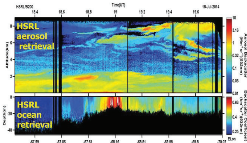
Figure 8.5. Backscatter from atmospheric aerosols and ocean particles as measured by an airborne 532 nm LiDAR along a transect line in the North Atlantic during a field program in 2014. Color codes indicate the intensity of scattering with red (high) and blue (low). SOURCE: Modified from Hair et al. (2016).
