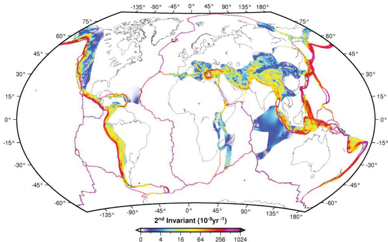
FIGURE 10.21 Color contours of the strain rate along the boundaries of the major tectonic plates derived from 22,500 GPS velocities. Most major earthquakes occur in these high strain rate areas, and so refined mapping is needed to improve the accuracy of the global earthquake hazard maps as well as to better understand the physics of plate boundaries as well as the extent and physics of intraplate deformation. SOURCE: Kreemer et al. (2014).
