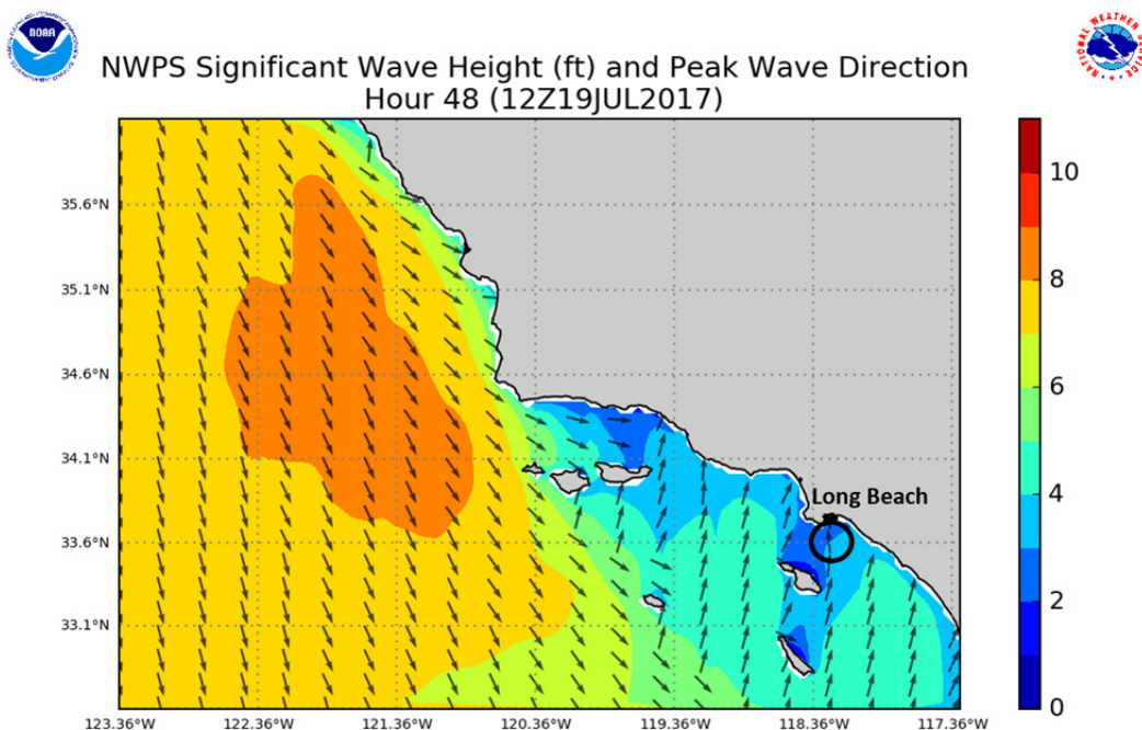
FIGURE 4.8 Nearshore Wave Prediction System (NWPS) model illustrating island sheltering and corresponding bi-modality of wave approach. Black circle at the Port of Long Beach represents the critical area of vessel transit during an energetic south swell. (Figure courtesy of NOAA/National Weather Service).
