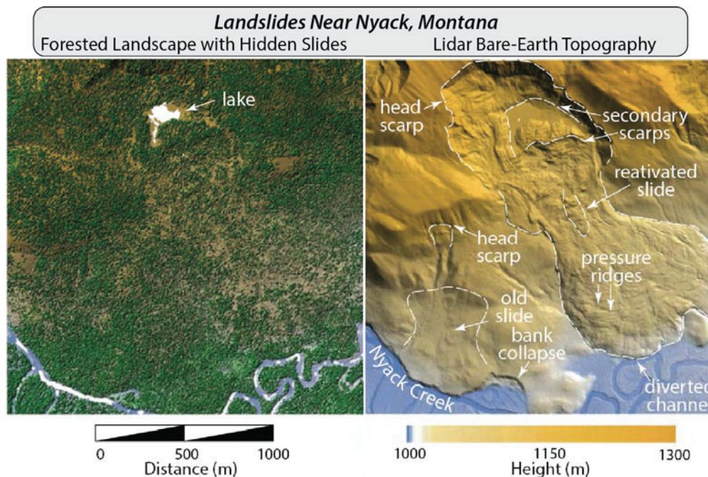
FIGURE 10.6 Discovering landslides, Nyack, Montana: the role of lidar bare-earth topography. (Left) Landsat/GoogleEarth image of the flank of Loneman Mountain. The isolated lake provides a clue to a topography disrupted by landslides. SOURCE: GoogleEarth. (Right) Lidar bare-earth, shaded relief topography exposes multiple generations of landslides with diverse modes of failure and movement, including mass flows, block rotations, and gravitational collapse. Back rotation in the headward area of the large slide ponded drainages and created the upland lake. Removal of vegetation and topographic resolution at \leq 1 m reveals nested slides, modes of mass movement, contrasts in surface roughness related to the relative sequence of landsliding, undercutting by and deflection of rivers, reactivation of older slides, and changes of channel geometry due to base-level changes by landslides. SOURCE: Data provided by Ramesh Shrestha and the National Center for Airborne Laser Mapping.
