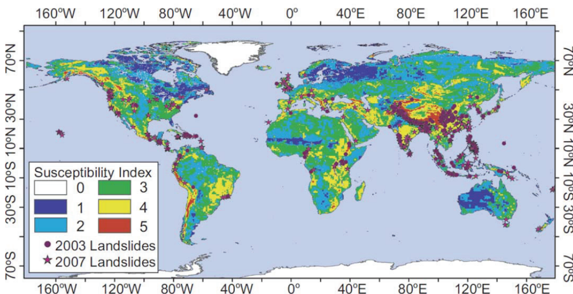
Figure 6.10. Global landslide susceptibility index (Hong et al., 2007) plotted with the 2003 and 2007 landslide inventory data. The index integrates slope land-cover change, geology, road presence, and operational nowcasts of landslide potential are made by checking whether 1-day, 3-day and 7-day precipitation intensity thresholds and accumulations are met. Further details and up-to-date forecasts are available at https://pmm.nasa.gov/precip-apps . Source: NASA
