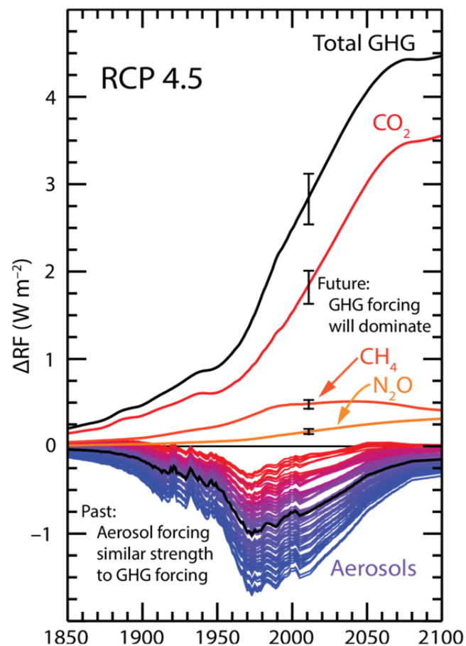
FIGURE 9-13: Time series of change in radiative forcing of climate ( \Delta RF ) due to CO_2 , CH_4 , N_2O , and all anthropogenic GHGs, from 1850 to 2100, based on the RCP 4.5 scenario (Meinshausen et al. 2011) (top) and 71 plausible scenarios for total \Delta RF due to anthropogenic aerosols (combination of the aerosol direct effect and the aerosol-cloud interaction) from Smith and Bond (2014) (bottom). Blue colors are used to denote the high end of the range of aerosol cooling (i.e., more overall cooling of climate) and red colors denote the low end (less overall cooling). Source: Salawitch, R. J., Canty, T. P., Hope, A. P., Tribett, W. R., & Bennett, B. F. (2017). Paris Climate Agreement: Beacon of Hope (1 ed.): Springer International Publishing. Figure 1.10. https://doi.org/10.1007/978-3-319-46939-3 . Creative Commons Attribution 4.0 International.
