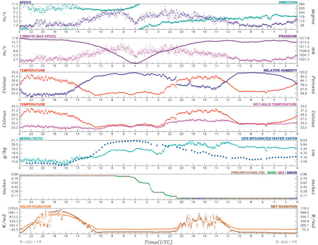
FIG. 5. Time series of surface meteorology parameters, integrated water vapor, solar radiation, and net radiation collected on a 10-m tower collocated with the Doppler wind profiler at New Bern, North Carolina, during the passage of Hurricane Arthur. Time proceeds from right to left along the horizontal axis.
