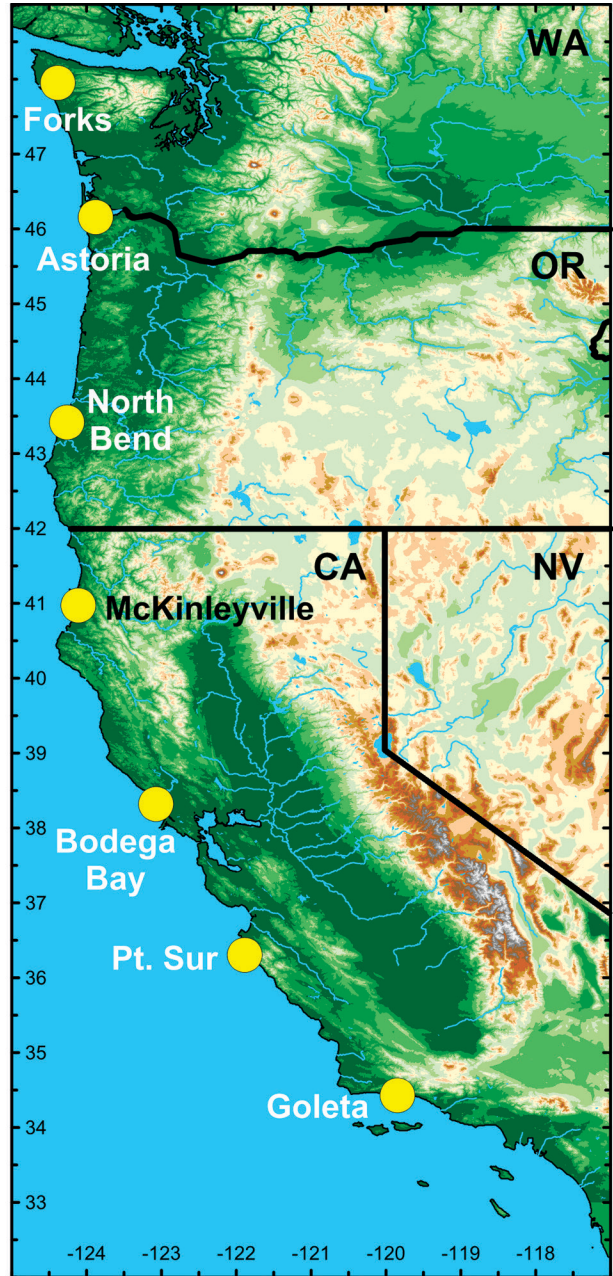
FIG. 3. Map of the U.S. West Coast showing the locations of seven semipermanent ARO deployments with 449-MHz wind profilers. This network is supported by the California Department of Water Resources and the Pacific Northwest National Laboratory.
