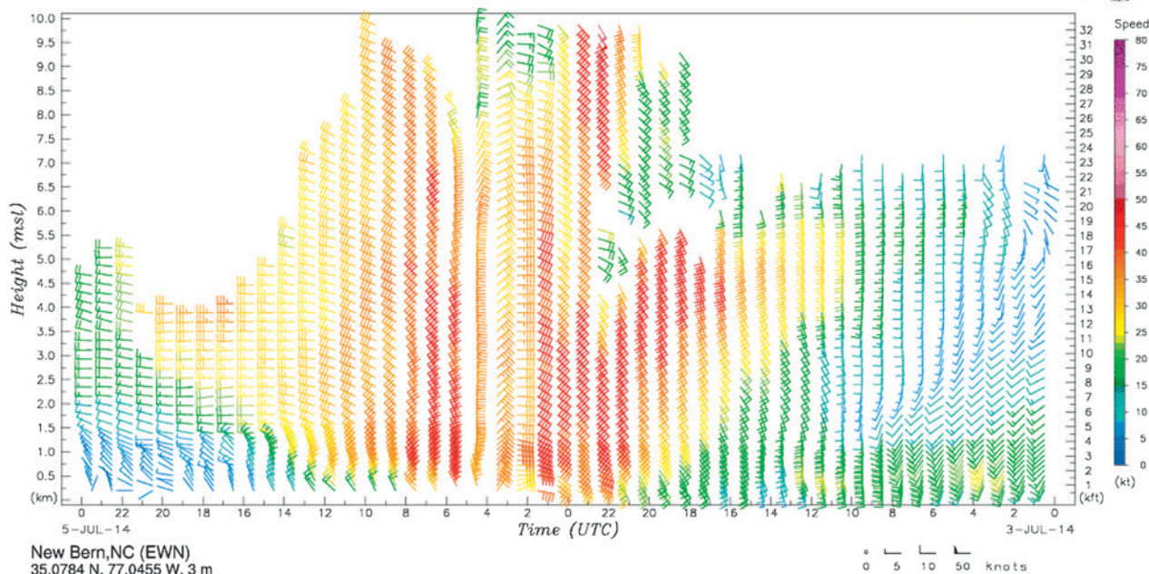
FIG. 4. 48-h time-height display of hourly-averaged wind profile observations collected at New Bern, North Carolina, during the passage of Hurricane Arthur. The wind speed at each level and time is denoted by the barb convention shown in the lower right-hand corner and is also color-coded to the speed scale on the right-hand side of the display. Wind direction is indicated by the direction from which the bottom of each flagpole is pointing. Time proceeds from right to left along the horizontal axis.
