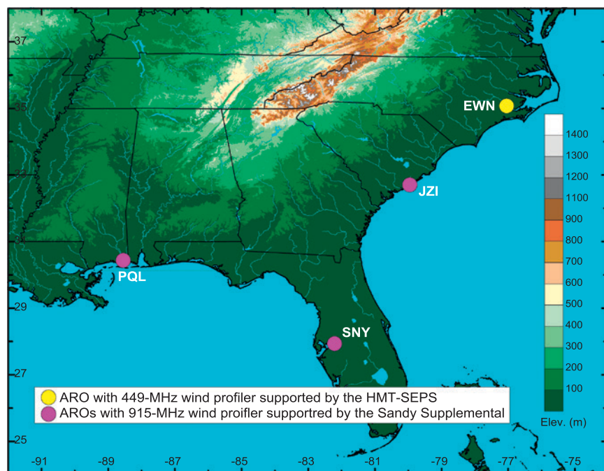
FIG. 2. Map of the southeast United States showing the locations and Station IDs (see Table 1) for the ARO deployments supported by the HMT-SEPS and Sandy Supplemental projects.
