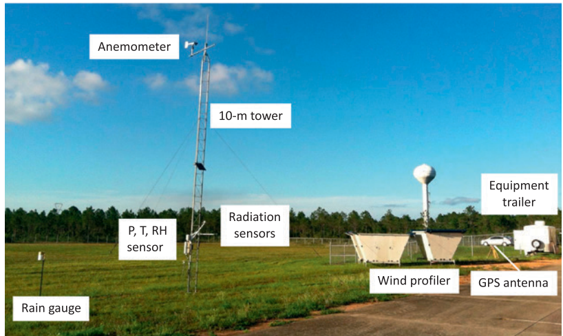
FIG. 1. A typical ARO deployment with a 915-MHz wind profiler. This ARO is installed in Moss Pt., Mississippi, as part of the Sandy Supplemental project.
