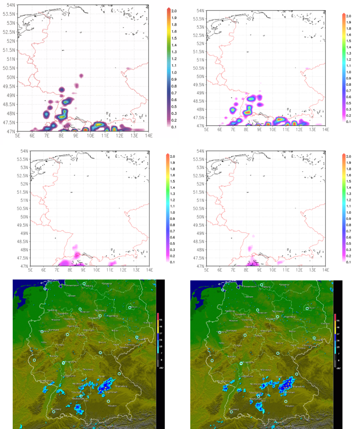
Figure 5: 15 minutes accumulated precipitation [mm] for different model physics compared qualitatively with the reflectivity of the radar composite of DWD at 00:30 UTC (left panel) and at 01:00 UTC (right panel) on August 14, 2007. Sigma diffusion (upper panel), modified horizontal diffusion (middle panel) and radar image (lower panel).
