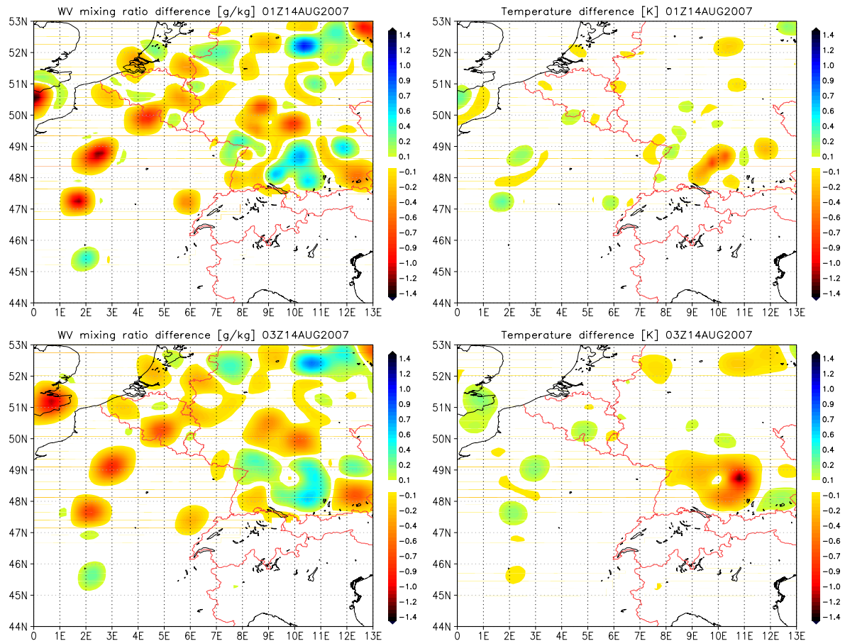
Figure 8: Difference between assimilation and no assimilation in water-vapor mixing ratio [g/kg] (left) and temperature [K] (right) in 850 hPa at 1 UTC (upper panel) and 3 UTC (lower panel) valid on August 14, 2007.
