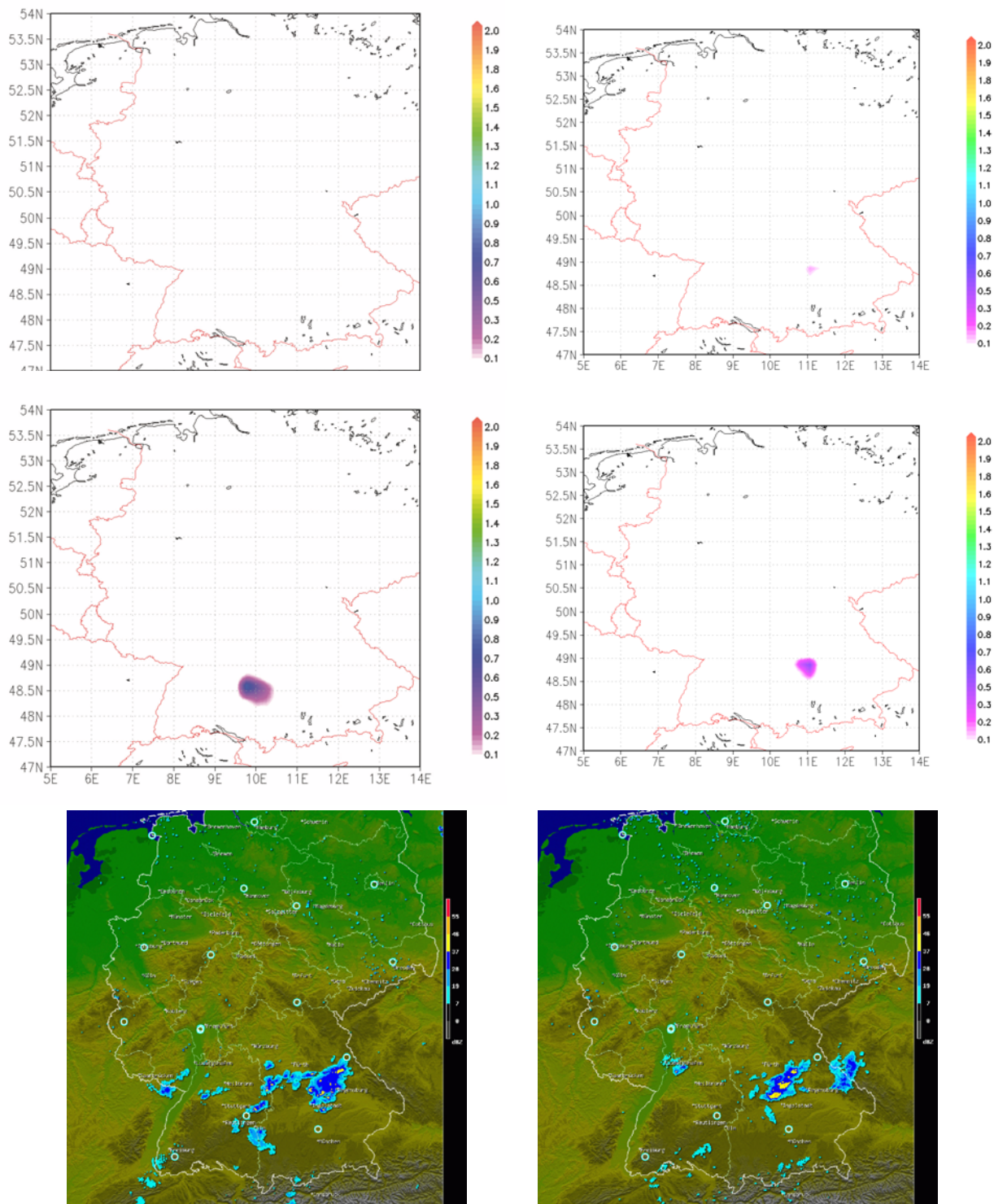
Figure 12: 15 min accumulated precipitation [mm] with and without assimilation compared qualitatively with the reflectivity of the radar composite of DWD at 01:30 UTC (left panel) and at 04:00 UTC (right panel) on August 14, 2007. No assimilation (upper panel), assimilation (middle panel) and radar image (lower panel).
