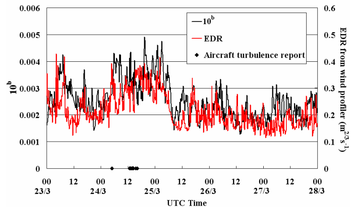
Figure 5. Time series of 10^b from the radiometer and EDR derived from Sha Lo Wan wind profiler for the period 23 to 28 March 2004. Aircraft reports of significant turbulence are marked on the time axis.
