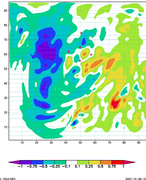
Figure 2: Sonde run temperature analysis increments (sonde-control) at hour 6 (12 UTC), at \sigma=0.533 . The model domain corresponds to the geographic area shown in Figure 1. The axes are labeled by gridpoint index, and the sonde data locations are shown as red crosses.
