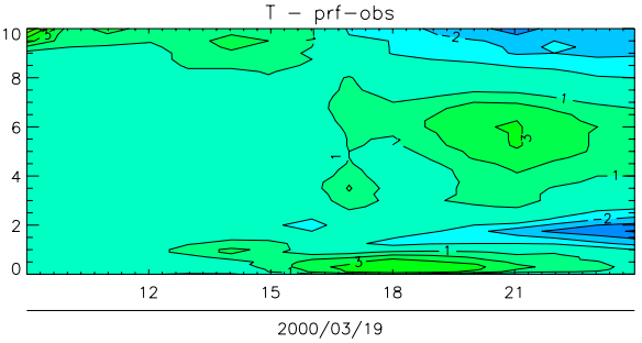
Figure 4: Time-height section of observed (top panel), simulated (center panel), and differences between simulated and observed (bottom panel) temperatures (K) at the microwave profiler location for the ARM control run.
