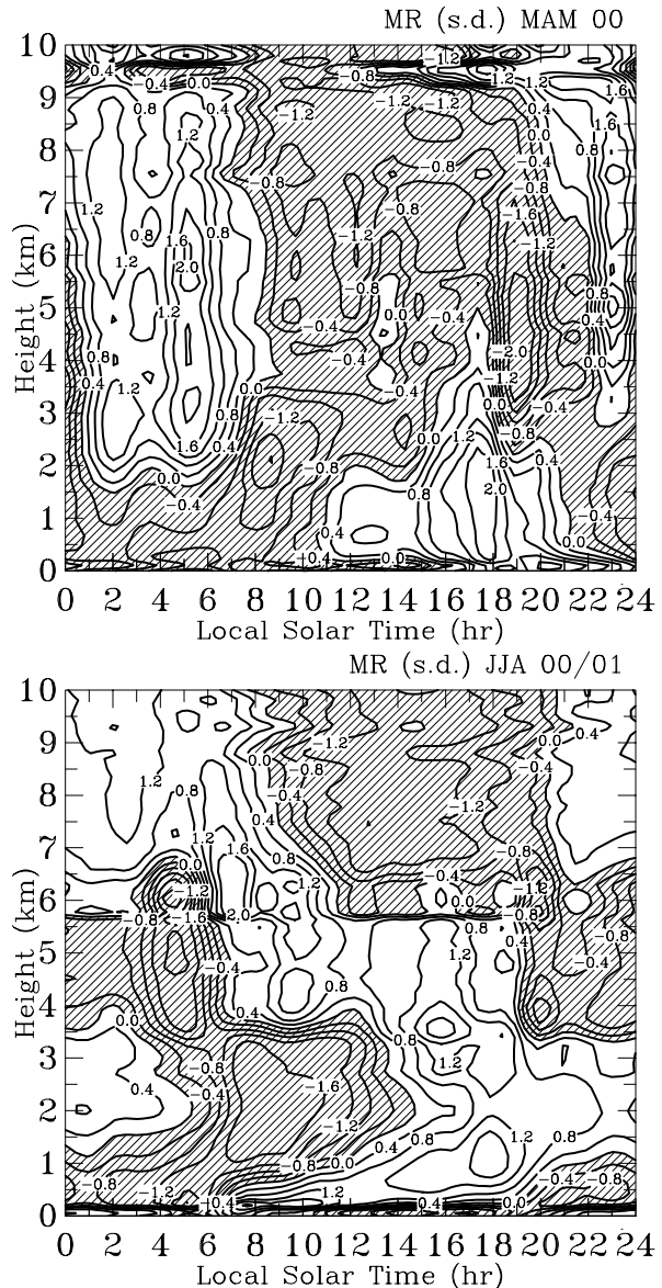
Figure 4. Seasonal-mean diurnal anomalies (normalized by diurnal standard deviation at each level) of atmospheric MR derived from MWRP data. Negative anomalies are hatched.
