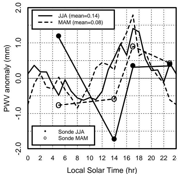
Figure 2. Diurnal variations of PW anomaly (mm) from MWRP and radiosonde data in 2000.
