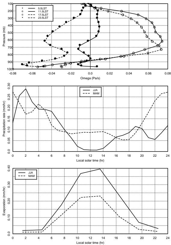
Figure 5. Omega profiles at 5.5, 11.5, 17.5, 23.5 LST in July from the 1975-1995 NCEP analysis data (a), diurnal variations of precipitation rate in JJA and MAM from the 1998-2000 SMOS data (b), and diurnal variations of surface evaporation in MAM and JJA from the 1994-1999 ARM IOP variational objective analysis data.
