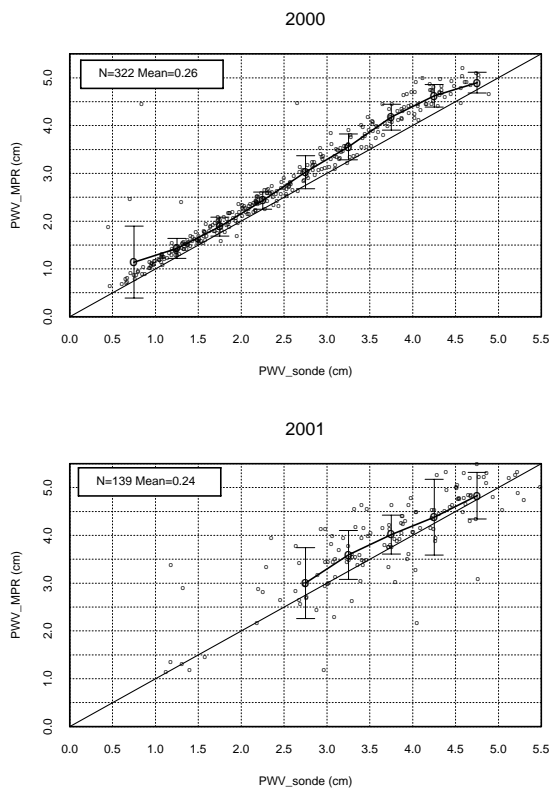
Figure 3. Comparisons of PW from coincident MWRP and radiosonde data in 2000 and 2001. Mean and standard deviation of MWRP-derived PW are also given as a function of radiosonde-measured PW.
