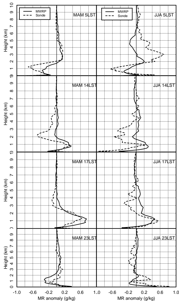
Figure 1. Comparisons of mean MR anomaly profiles from MWRP and radiosonde data at 5, 14, 17, and 23 LST in MAM and JJA in 2000.
