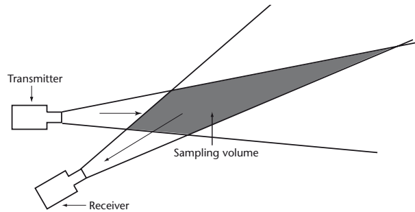
Figure 9.4. Visibility meter measuring back scatter
