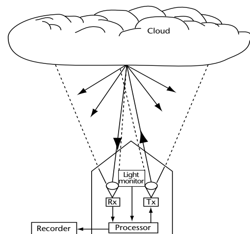
Figure 15.1. Typical laser ceilometer
