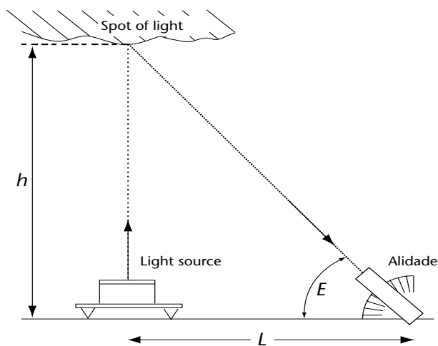
Figure 15.3. Principle of the cloud searchlight method
