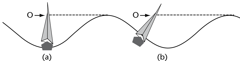
Figure 4.2. The effect of the ship's roll on the estimation of wave height
