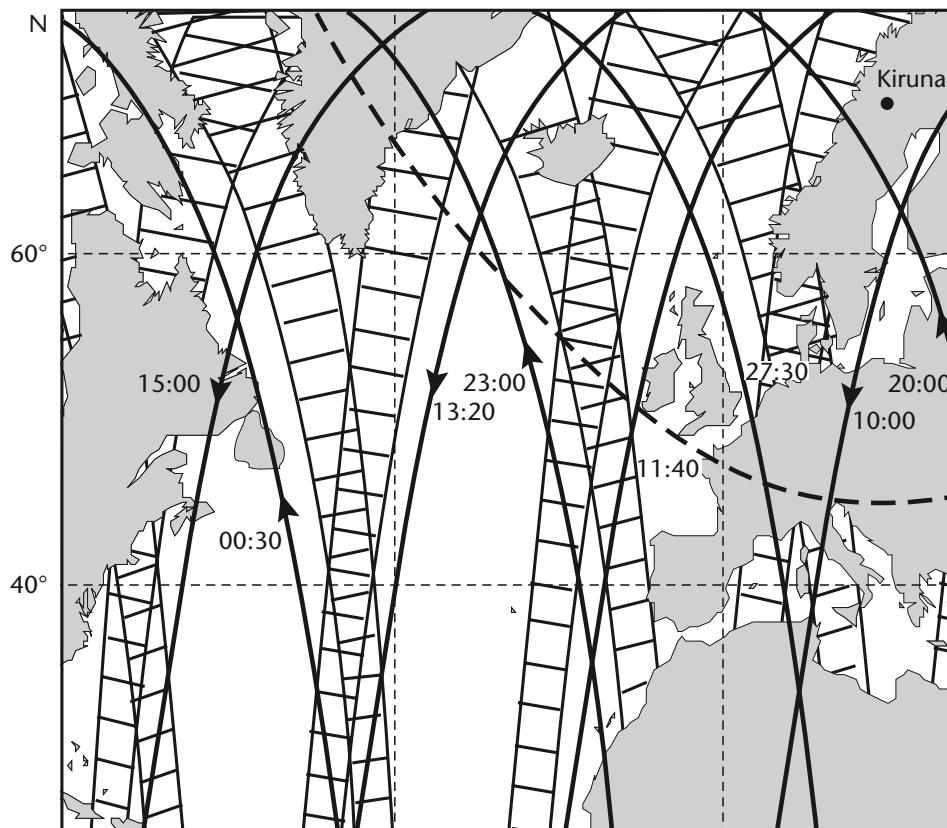
Figure 8.14. ERS-1 subsatellite tracks and wind scatterometer coverage of the North Atlantic region over one day. The large gaps are partially filled on subsequent days; nominally this occurs in a three-day cycle. The dashed lines show the limits of reception for the Kiruna ground station in Sweden.
