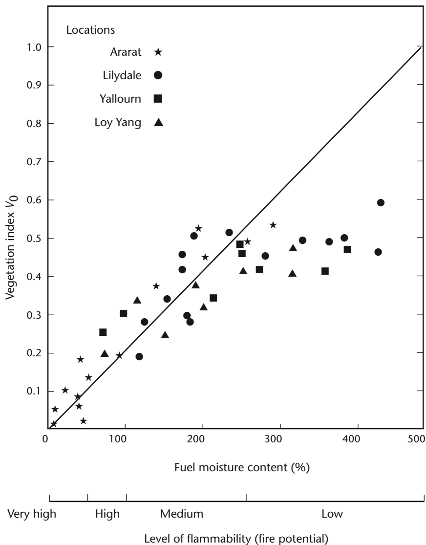
Figure 8.15. Full-cover, satellite-observed vegetation index as a function of fuel moisture content. Each point is a particular location average at a particular sampling time (see text).
