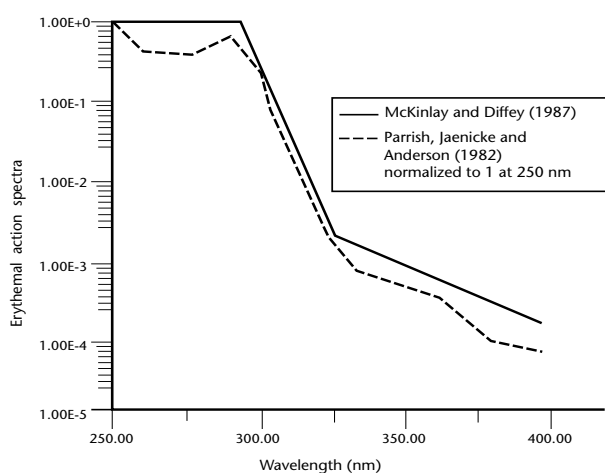
Figure 7.4. Erythemal curves as presented by Parrish, Jaenicke and Anderson (1982) and McKinlay and Diffey (1987)
