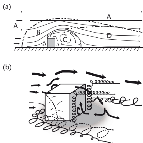
Figure 11.5. Typical two-dimensional flow around a building with flow normal to the upwind face (a): streamlines and flow zones; A represents undisturbed, B represents displacement, C represents cavity, D represents wake (after Halitsky, 1963), and (b): flow, and vortex structures (simplified after Hunt and others, 1978).
