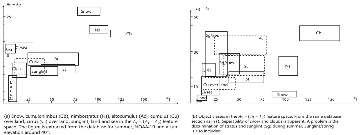
Figure 8.12. Identification of cloud and surface properties
