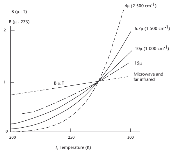
Figure 8.5. Temperature dependence of the Planck function
