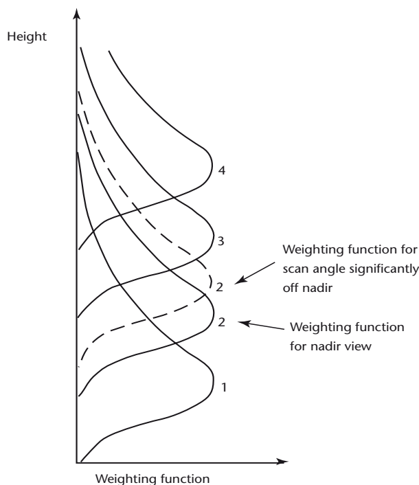
Figure 8.8. Schematic illustration of a group of weighting functions for nadir viewing and the effect of scanning off nadir on one of these functions
