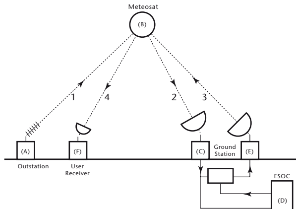
Figure 8.17. The METEOSAT DCP telemetry system
