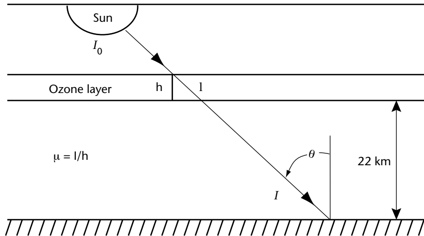
Total ozone by spectrophotometer
