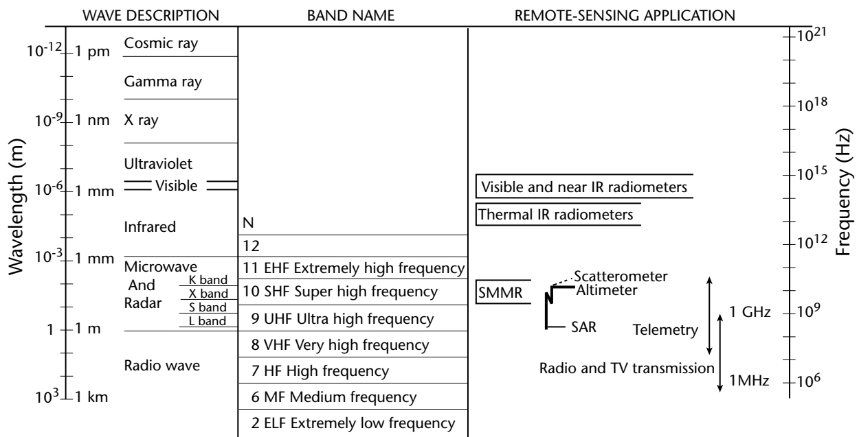
Figure 8.2. The electromagnetic spectrum showing some band definitions and typical remote-sensing applications
