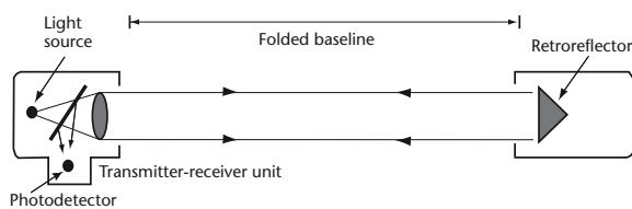
Figure 9.3. Single-ended transmissometer
