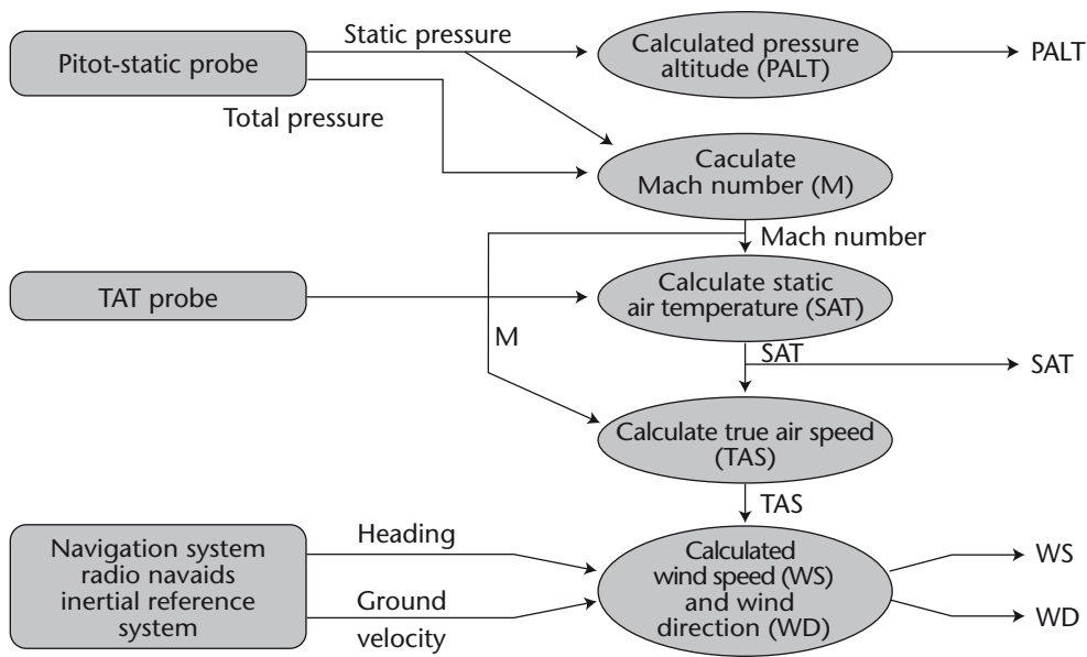
Figure 3.1. AMDAR sensor data processing
