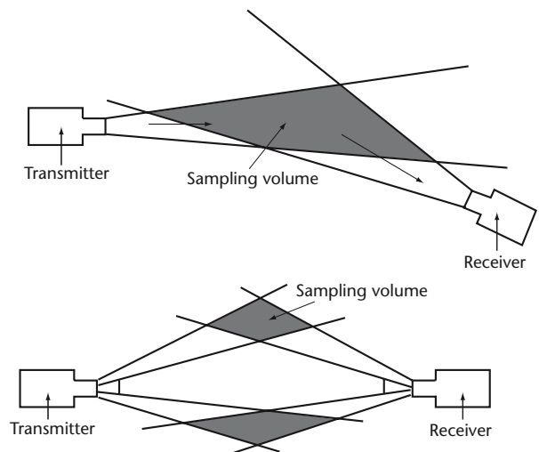
Figure 9.5. Two configurations of visibility meters measuring forward scatter
