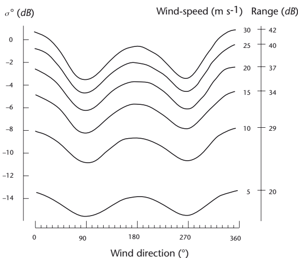
Figure 8.13. Measured backscatter, \sigma^0 (in decibels), against relative wind direction for different wind speeds. Data are for 13 GHz, vertical polarization.
