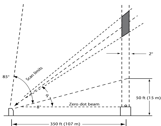
Figure 15.2. A typical rotating-beam ceilometer
