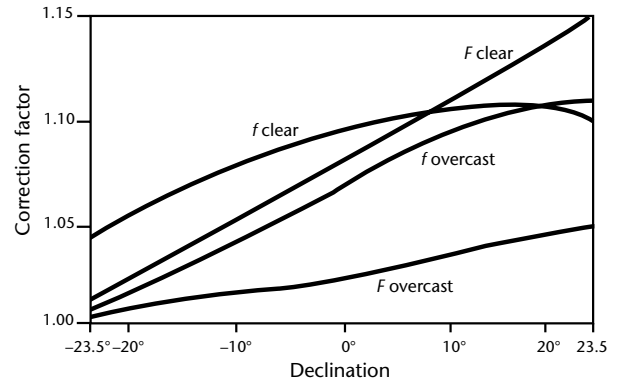
Comparison of calculated and empirically determined correction factors for a shading ring, with b/r = 0.169 ; f indicates calculated curves and F indicates empirical ones (after Dehne, 1980).
