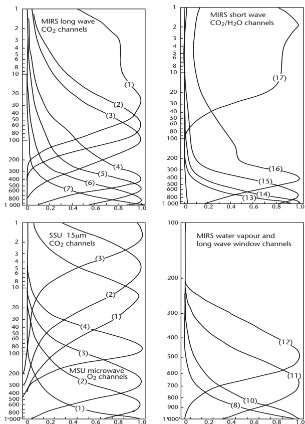
Figure 8.7. TOVS weighting functions (normalized)
