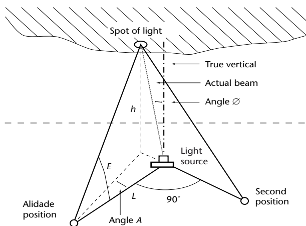
Figure 15.4. Checking the verticality of the searchlight beam
