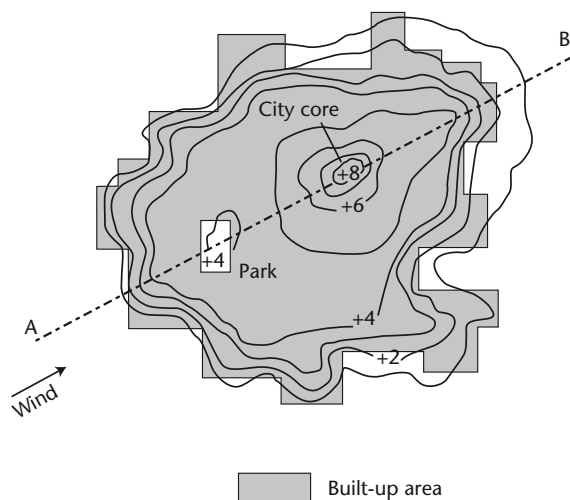
Figure 11.3. Typical spatial pattern of isotherms in a large city at night with calm, clear weather illustrating the heat island effect (after Oke, 1982).
