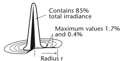
(a) The irradiance profile of the airy diffraction pattern
