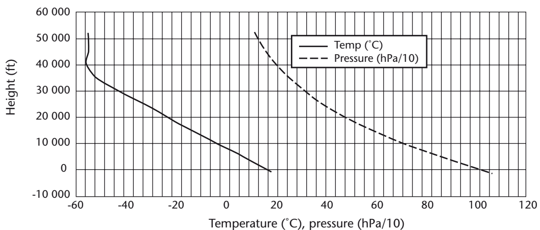
Figure 3.3. ICAO Standard Atmosphere
