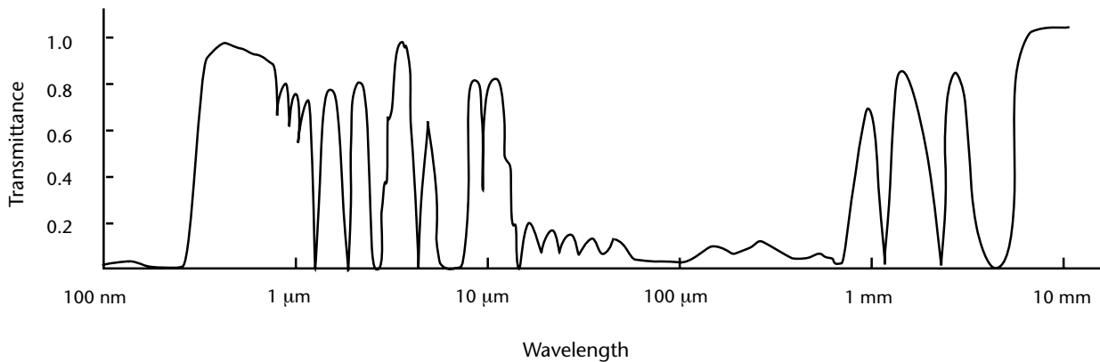
Figure 8.3. Appropriate transmittance of electromagnetic waves through the atmosphere
