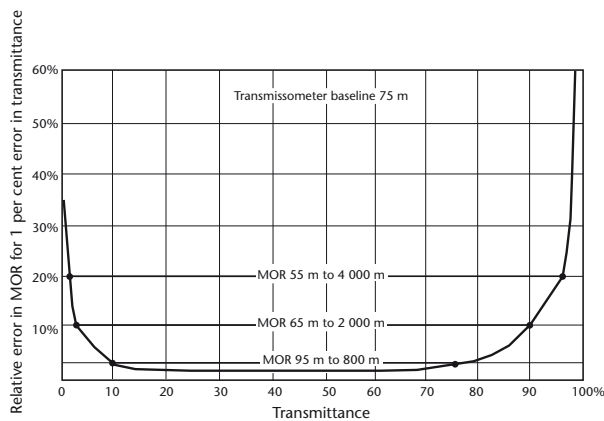
Figure 9.7. Error in measurements of meteorological optical range as a function of a 1 per cent error in transmittance
