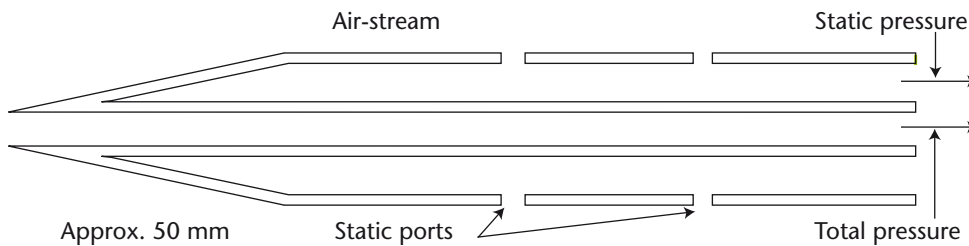
Figure 3.2. Pitot-static probe
