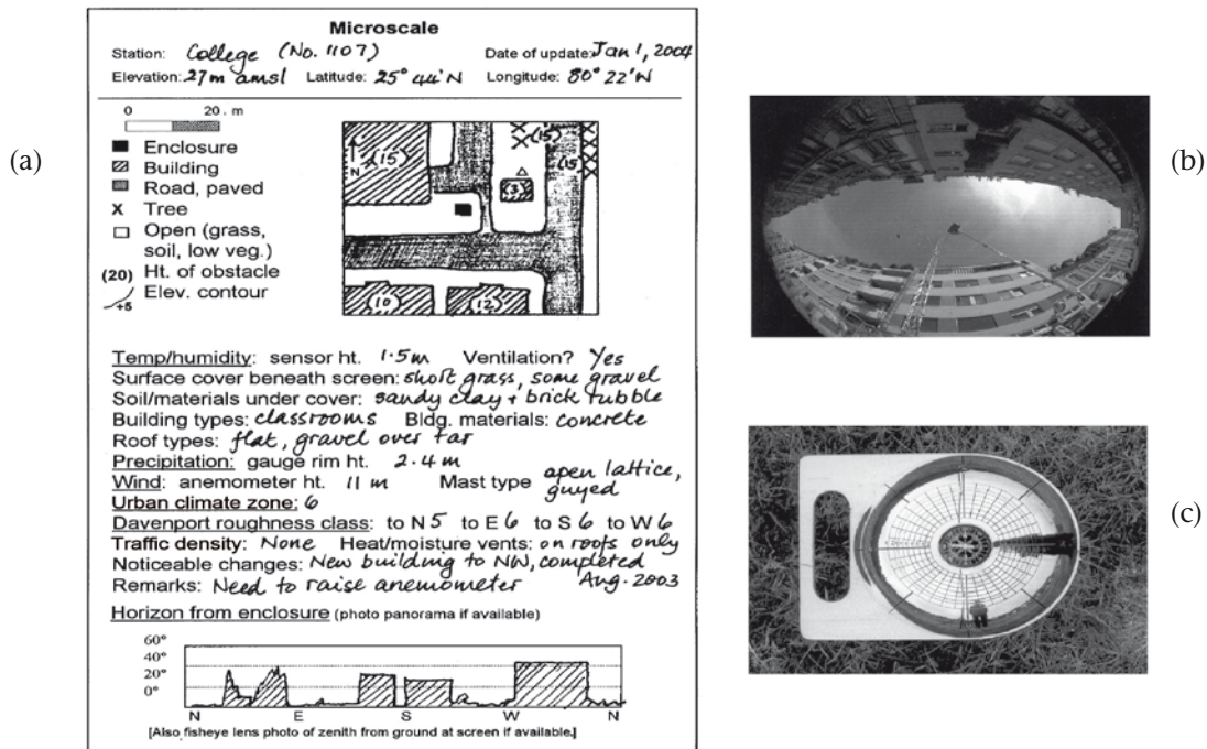
Figure 11.7. Information required to describe the microscale surroundings of an urban climate station; (a) a template for a metadata file; (b) an example of a fisheye lens photograph of a street canyon illustrating horizon obstruction; and (c) a UK Met Office hemispheric reflector placed on a rain gauge.
