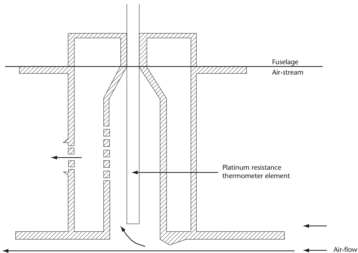
Figure 3.4. Aircraft thermometer probe
