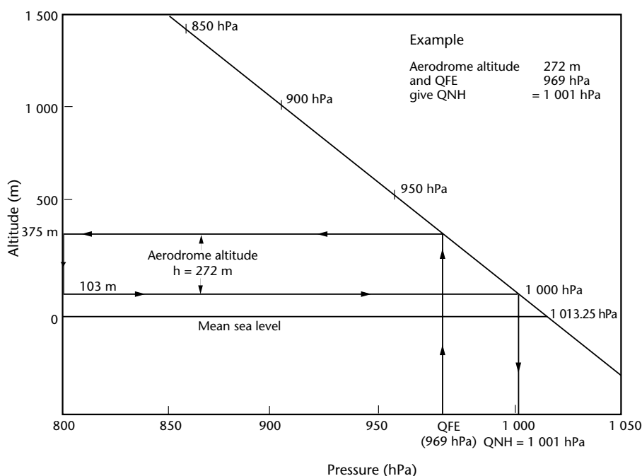
The relation between QFE and QNH
