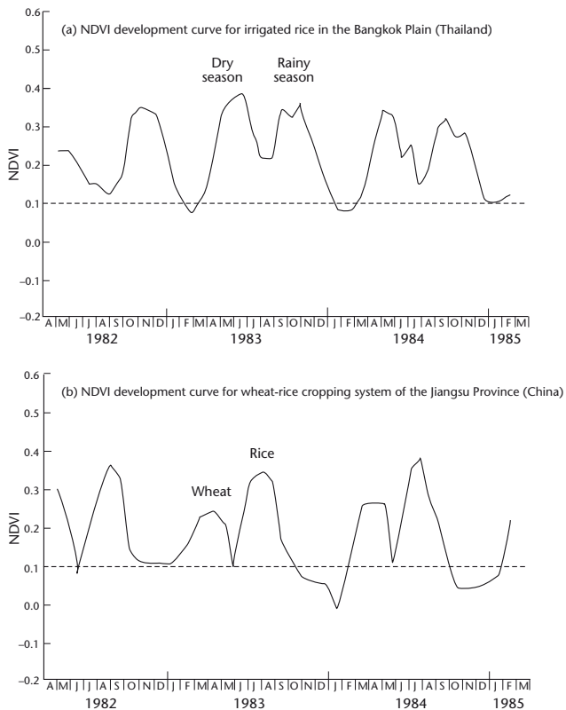
Figure 8.16. NDVI development curves for irrigated rice in Thailand and wheat-rice in China
