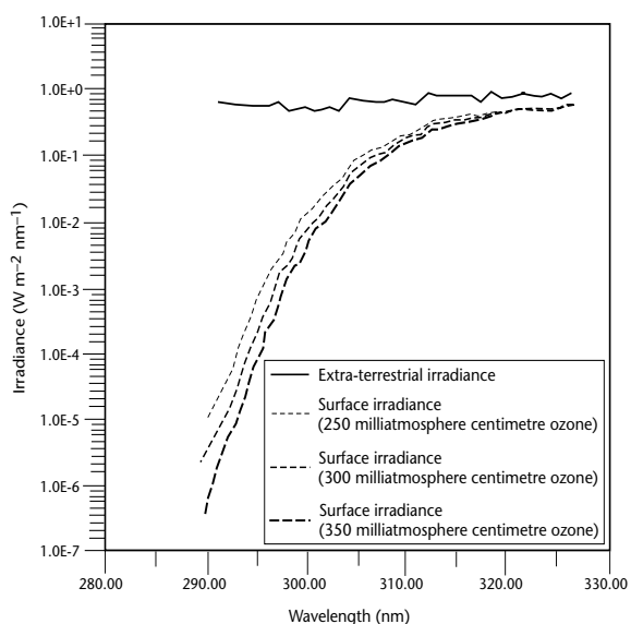
Figure 7.3. Model results illustrating the effect of increasing ozone levels on the transmission of UV-B radiation through the atmosphere
