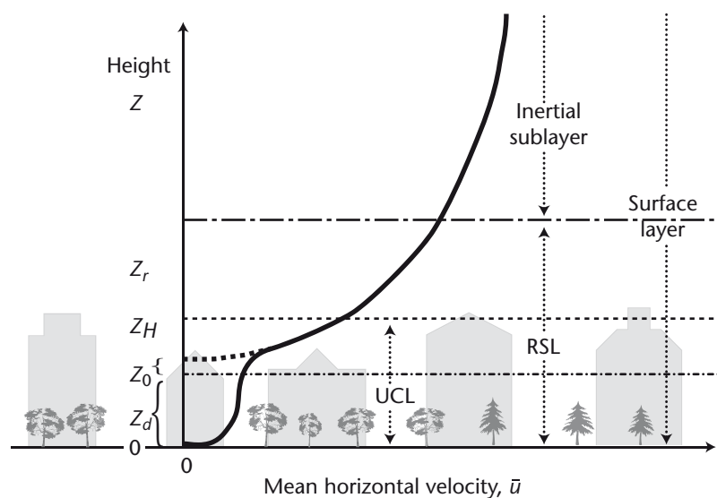
Figure 11.4. Generalized mean (spatial and temporal) wind velocity ( u ) profile in a densely developed urban area including the location of sublayers of the surface layer. The measures on the height scale are the mean height of the roughness elements ( z_H ) the roughness sublayer ( z_r , or the blending height), the roughness length ( z_0 ) and zero-plane displacement length ( z_d ). The dashed line represents the profile extrapolated from the inertial sublayer, the solid line represents the actual profile.
