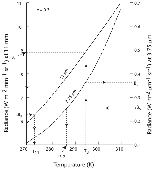
(a) The effect of semi-transparent cloud on radiances.
