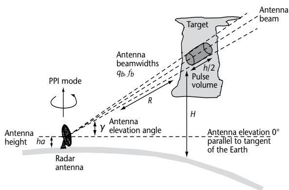
Figure 9.1. Propagation of electromagnetic waves through the atmosphere for a pulse weather radar; h_a is the height of the antenna above the Earth's surface, R is the range, h is the length of the pulse, h/2 is the sample volume depth and H is the height of the pulse above the Earth's surface
