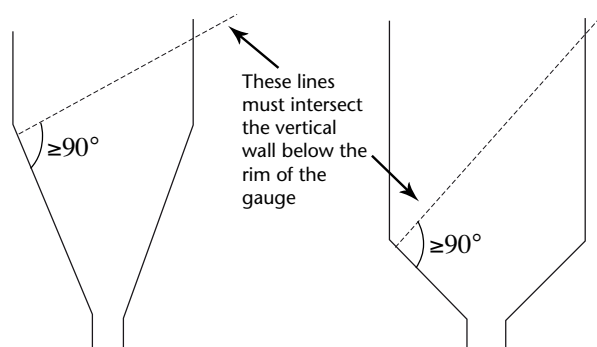
Figure 6.2. Suitable collectors for rain gauges
