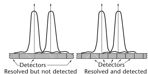
Figure 8.6. Optical resolution
