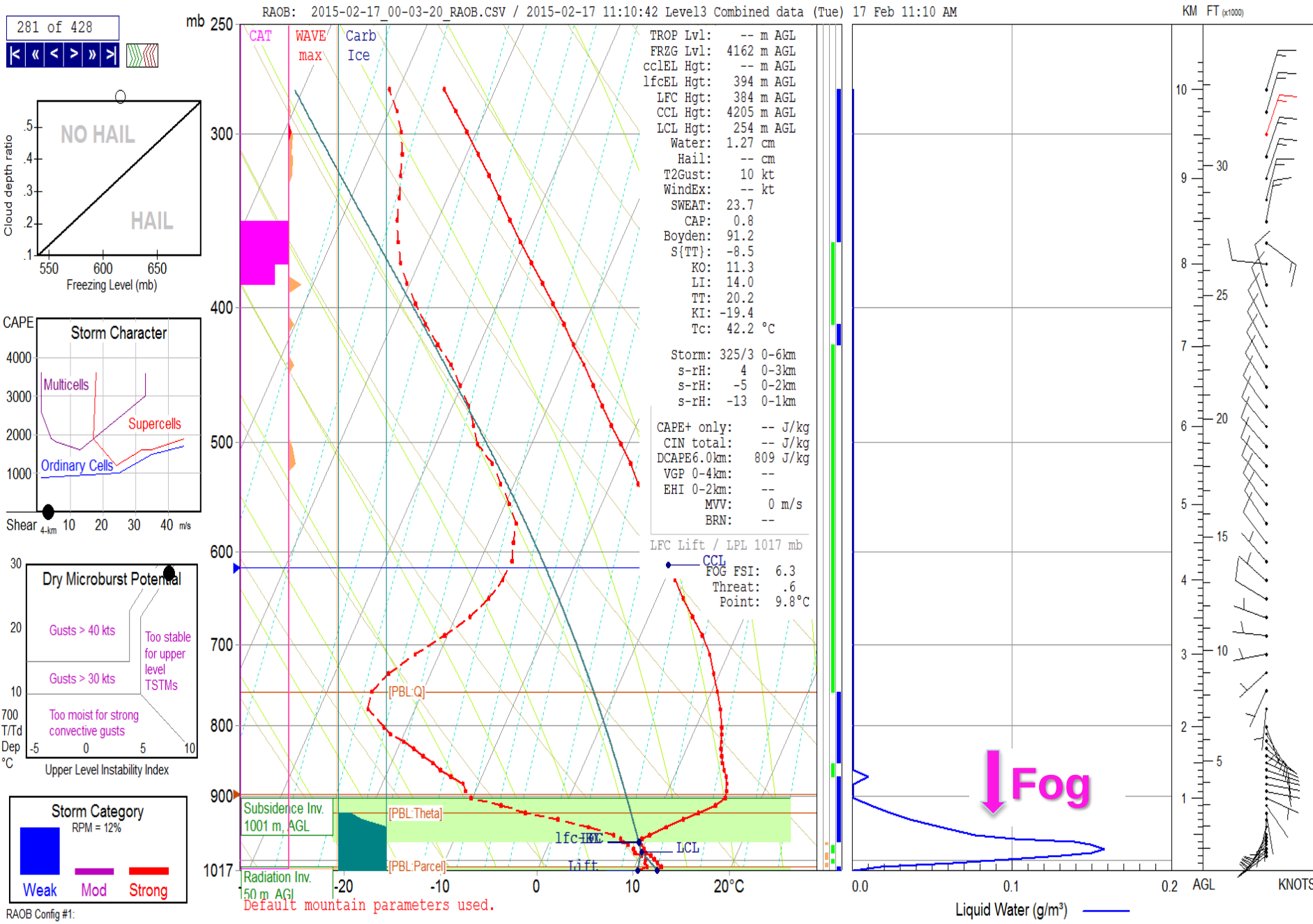
Sigma Sounding (1DVAR -- radiometer + analysis) at San Francisco, 11:10Z 17Feb15
